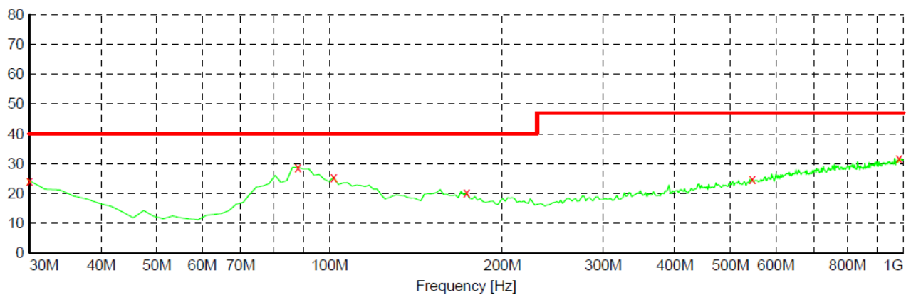
Level [dBμV/m]
